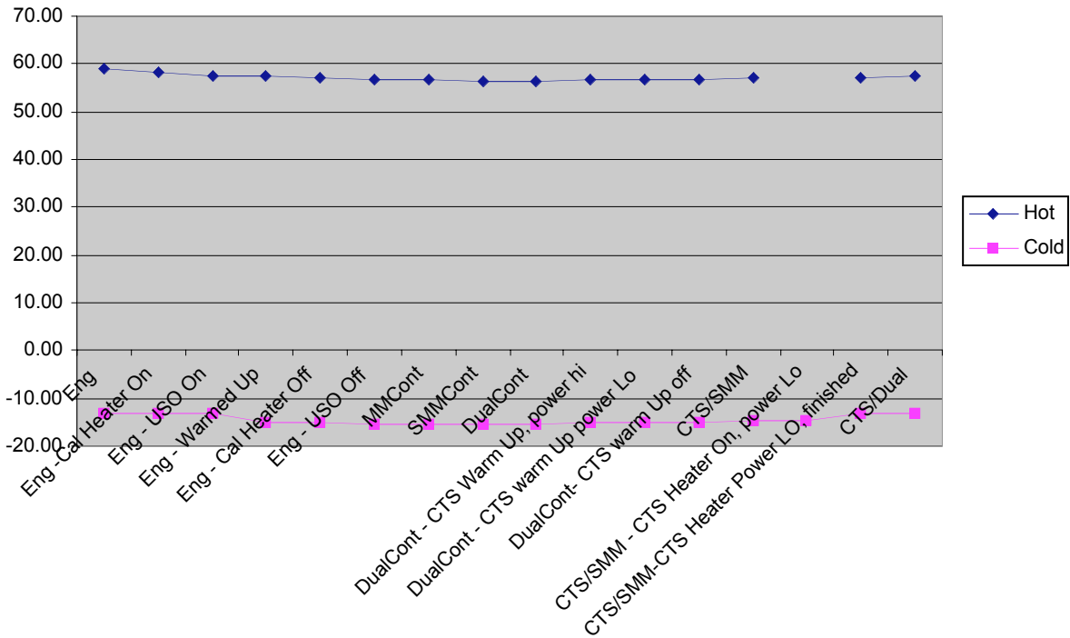
Sensor Electronics Temp
