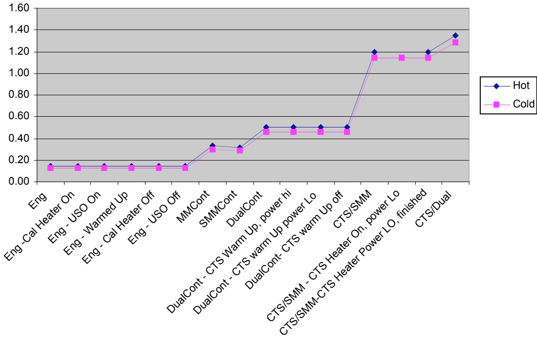
5V Current SBEU [A]
