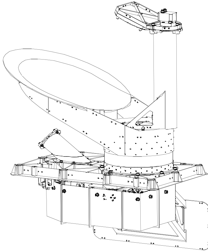
Figure 2.1-2: Sensor Unit
