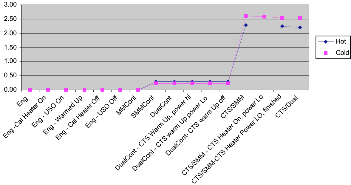
SMM PLL Error [V]
