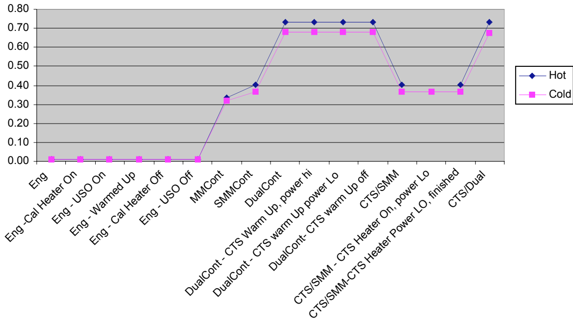
12V-2 Current SBEU [A]
