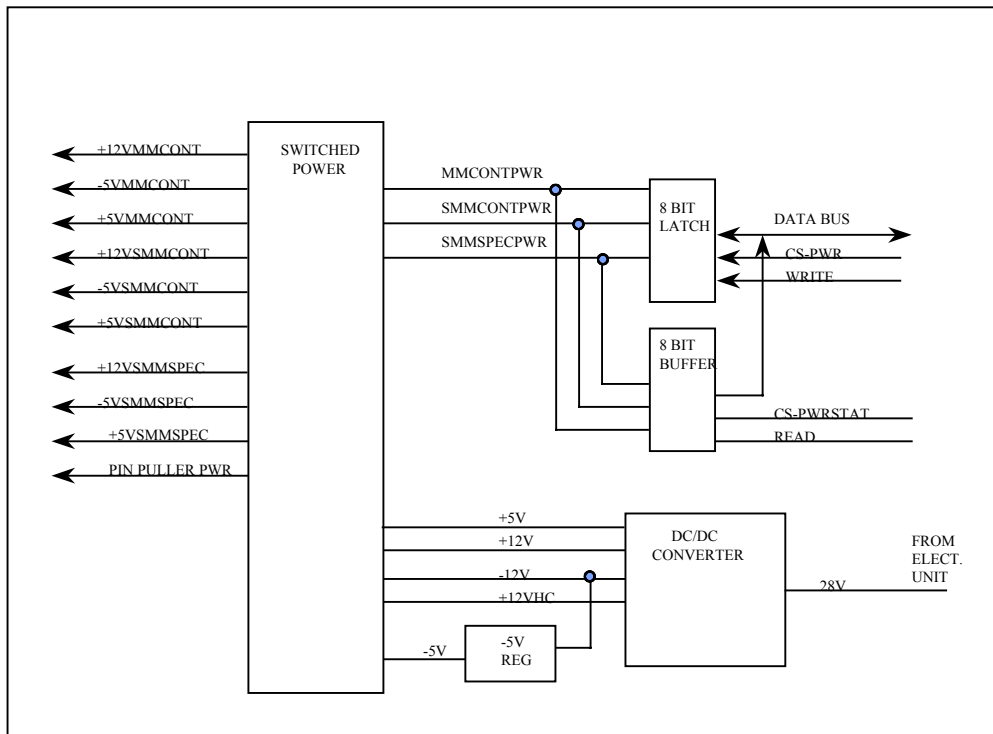
Fig. 2.3.1-2: Power Distribution Block Diagram (Sensor Backend Electronics Unit)
