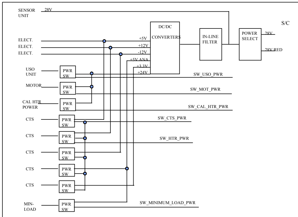
Fig. 2.3.1-1: Power Distribution Block Diagram (Electronics Unit)
