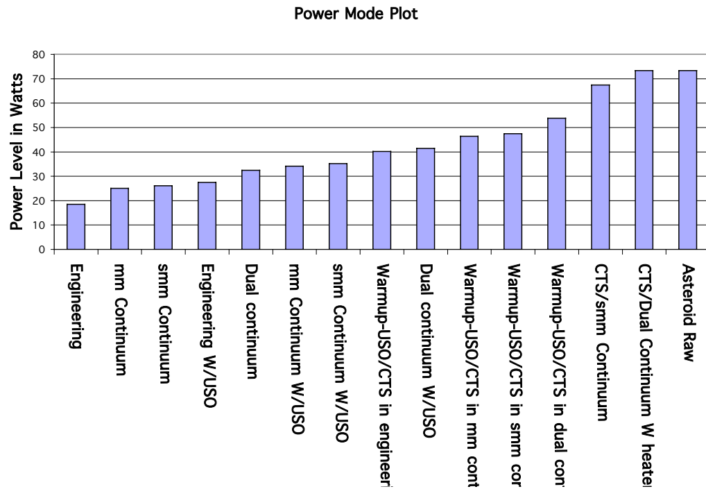
Figure 2.5.2-1: MIRO Instrument Operating Power (in watts)
