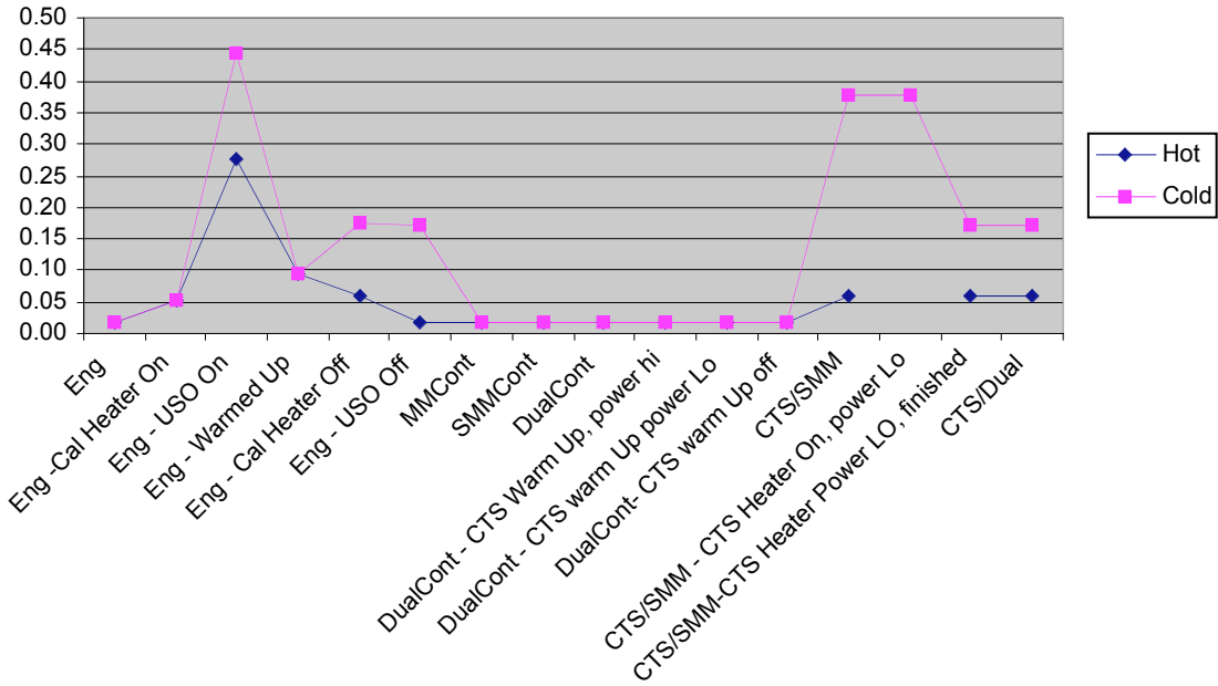
24V Current EU [A]
