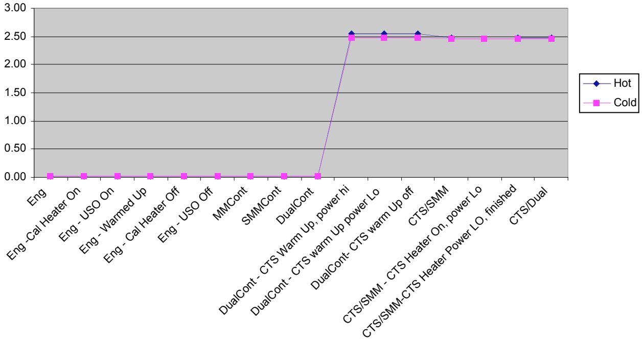
CTS V Ana 2 [V]
