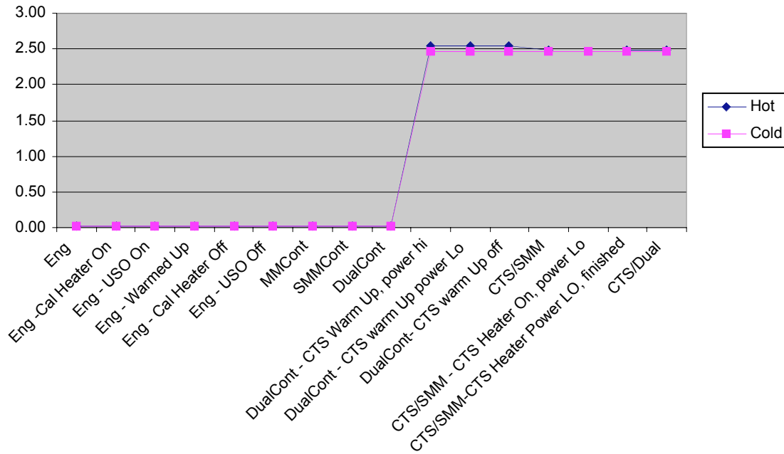
CTS V Ana1 [V]
