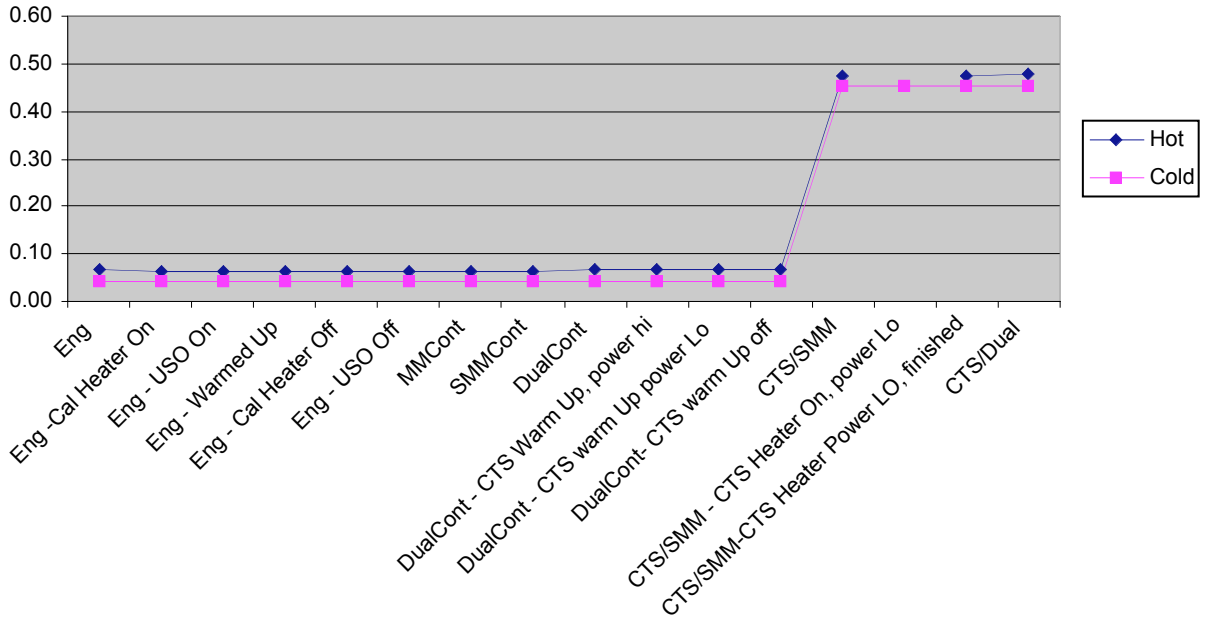
12V-1 Current SBEU [A]
