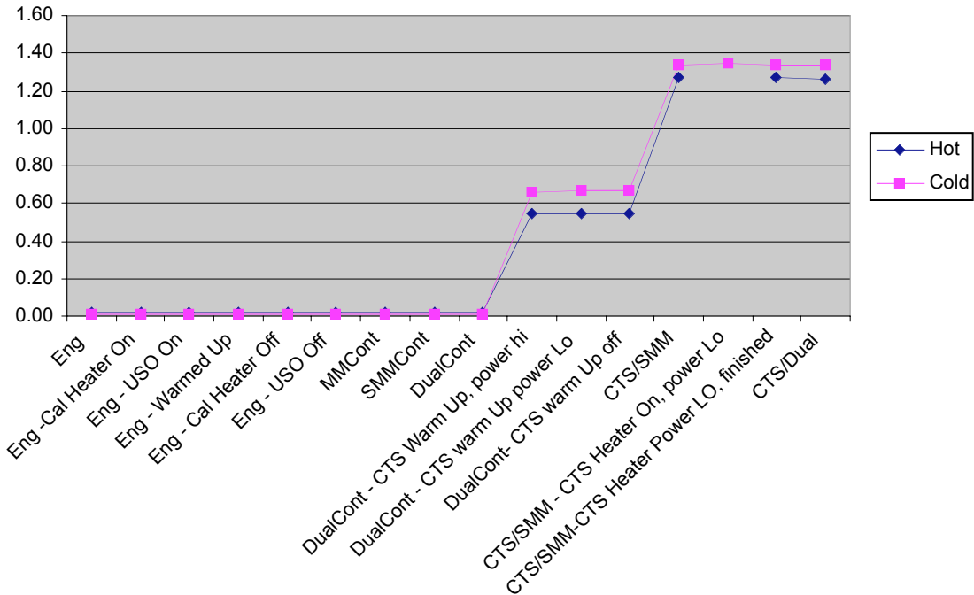
3.3V Current EU
