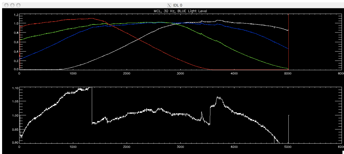
Figure 5. The 1-D individual lamp positions that made up the blue filter flat field. The feature near column 3700 is seen in all the images with flux in that region.
