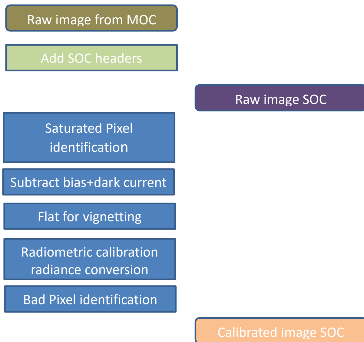
Figure 1. Graphical overview of the LICIAcube Payloads image calibration pipeline.
